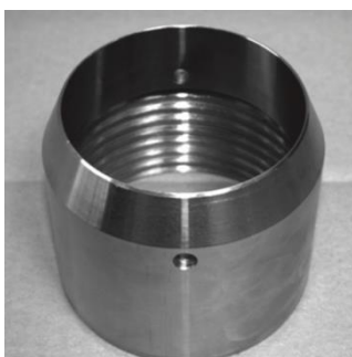
702003 Cutting shoe Ø 100 mm with O-Ring O-Ring inside O-Ring dseals against the cutting shoe of the liner probe
